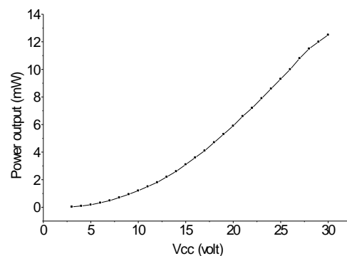
Fig.6: Variation of Power output with collector supply.
