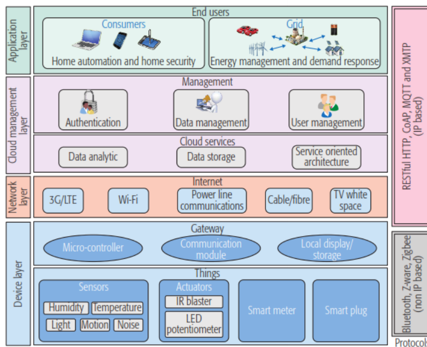
Figure 1. The system architecture of IoT [3].
