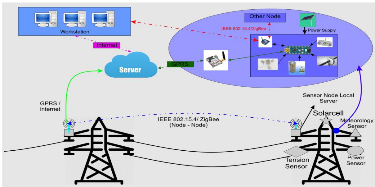
Figure 3. Transmission system based IoT.
