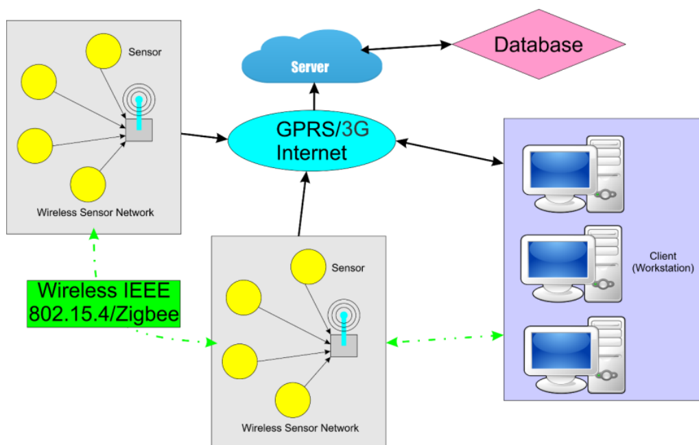
Figure 2. IoT system architecture.
